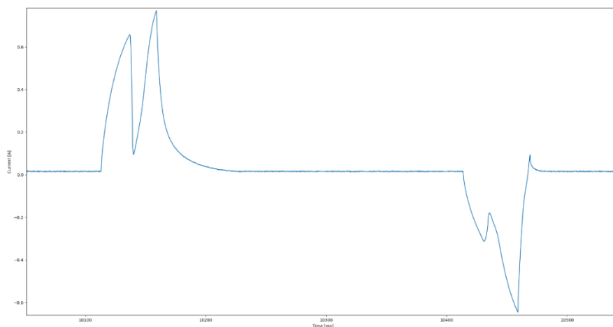
Figure 1: Current Flow during Actuation of a Latch Valve from Close to Open to Close
